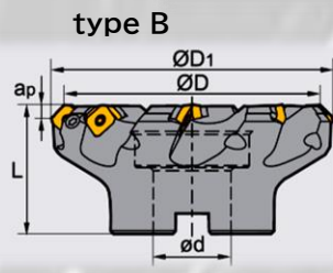
Face milling
